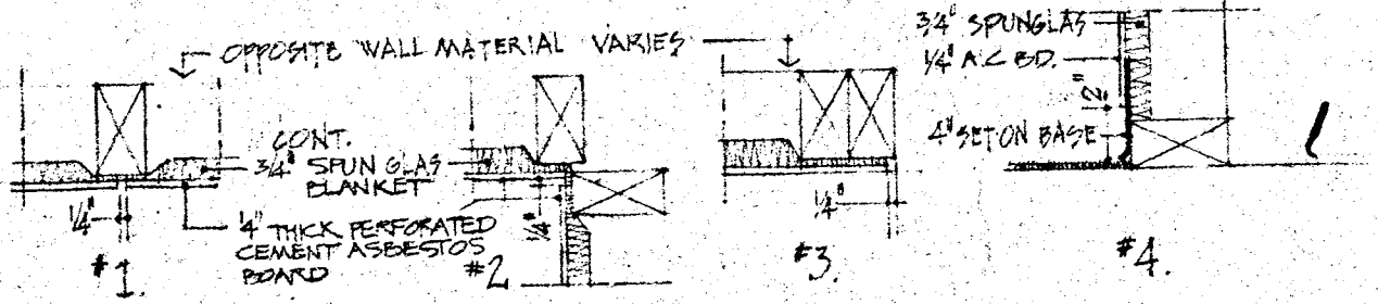
TYP. PEG BOARD DETAILS. SCALE 1/2" = 1'-0"
